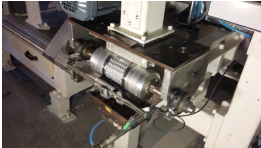
Metric SAP dosing unit ( 1-15g/ baby diaper)
