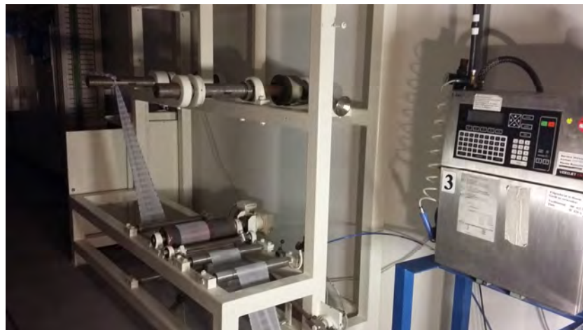
Frontal tape unwinder
